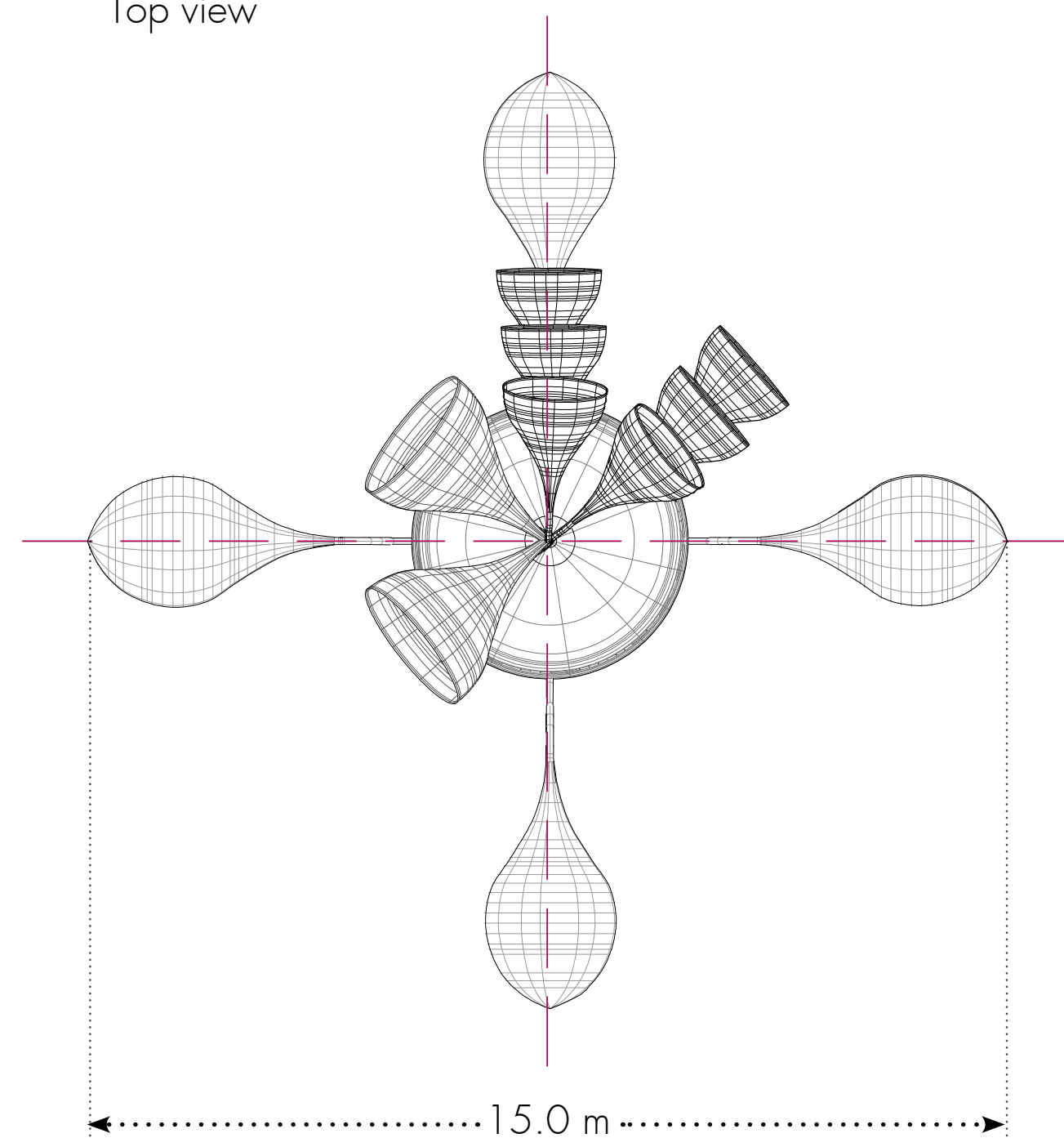
Water Hyacinth A Top view
