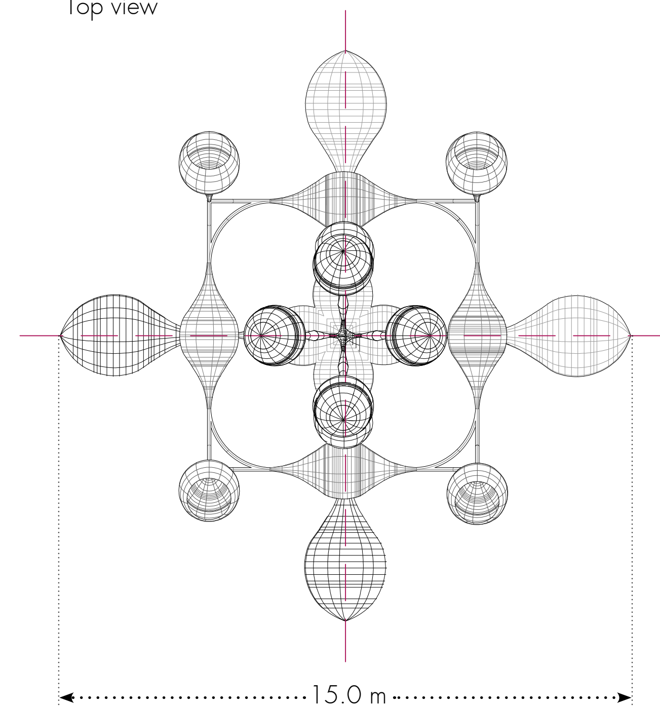
Water Hyacinth B Top view
