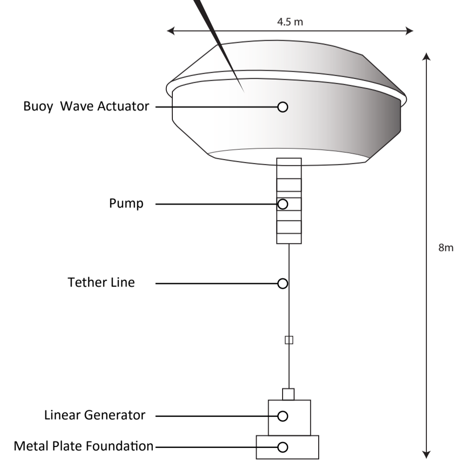
buoyant actuators the buoys harness the motion of waves off the coast and use it to create electricity and desalinate water.
