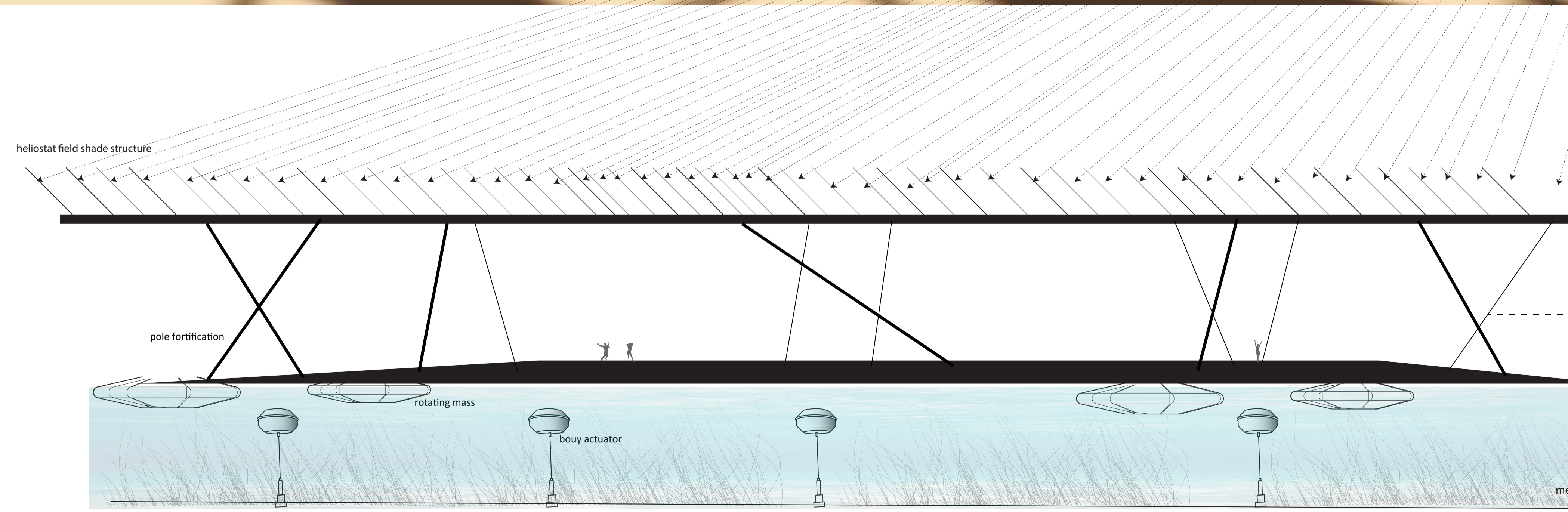
buoyant actuators the buoys harness the motion of waves off the coast and use it to create electricity and desalinate water.
